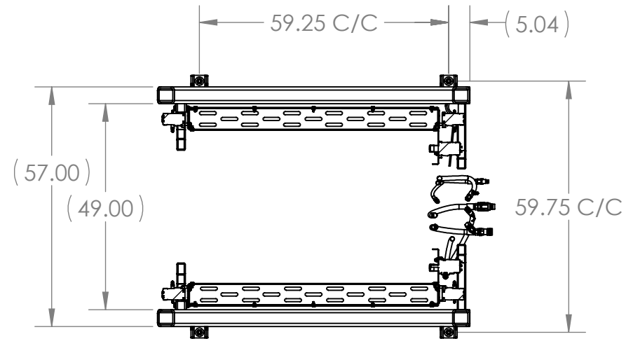
SECTION A-A (SOME COMPONENTS HIDDEN FOR CLARITY)
