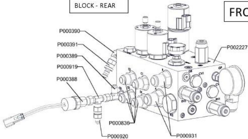
BLOCK - REAR
