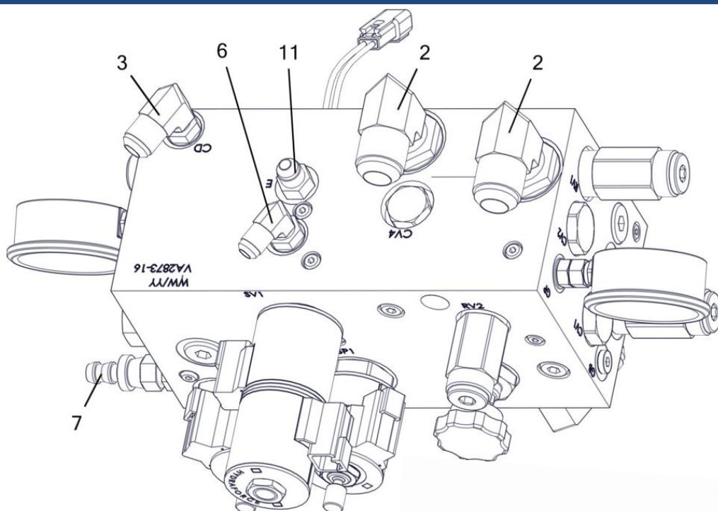
Hydraulic Block - Non-Fan Side View
